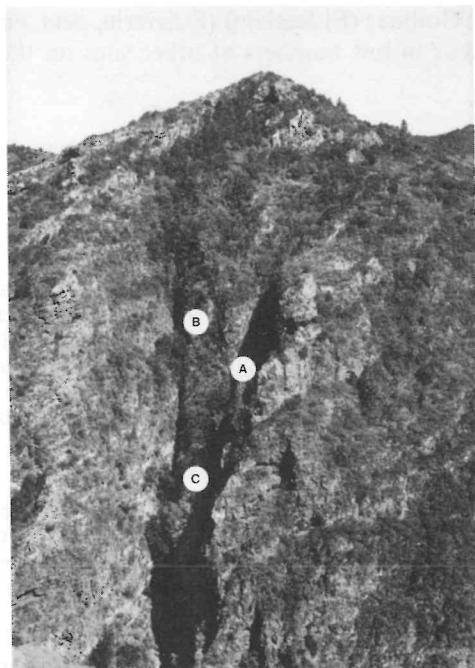
Fig. 1: General view of the breeding area of Puffinus puffinus in the Barranco de Los Cochinos (Tenerife). Point "A" indicates the location of the colony discovered while points "B" and "C" refer to possible breeding sites.
